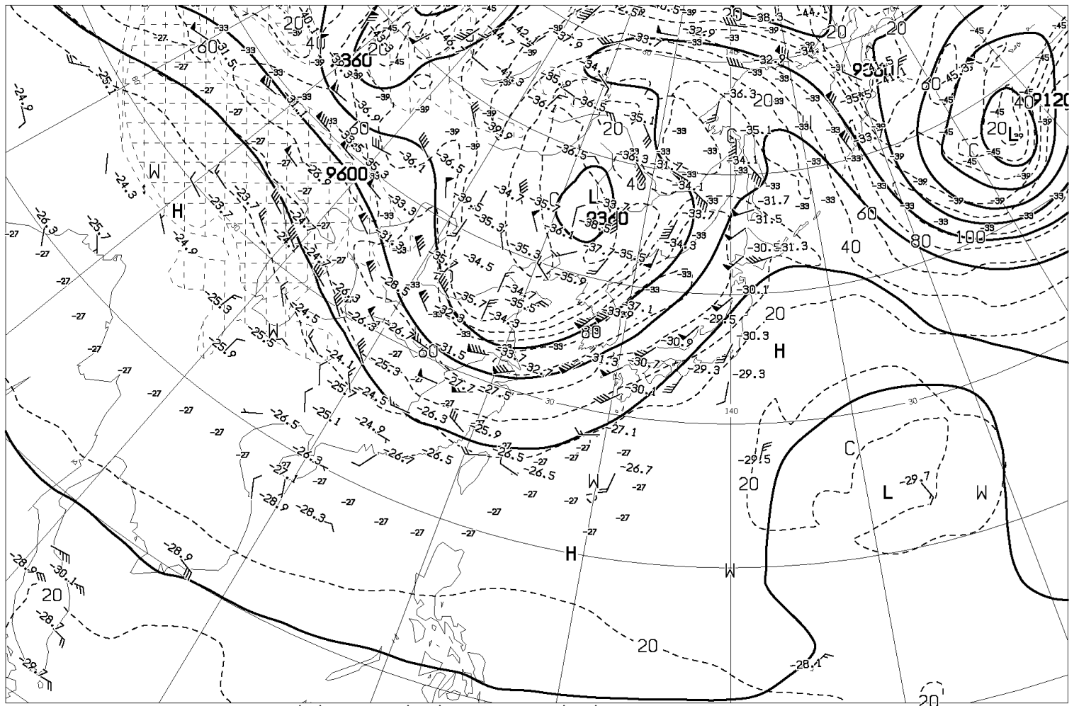
ANALYSIS 300hPa: HEIGHT(M), TEMP(°C), ISOTACH(KT)
