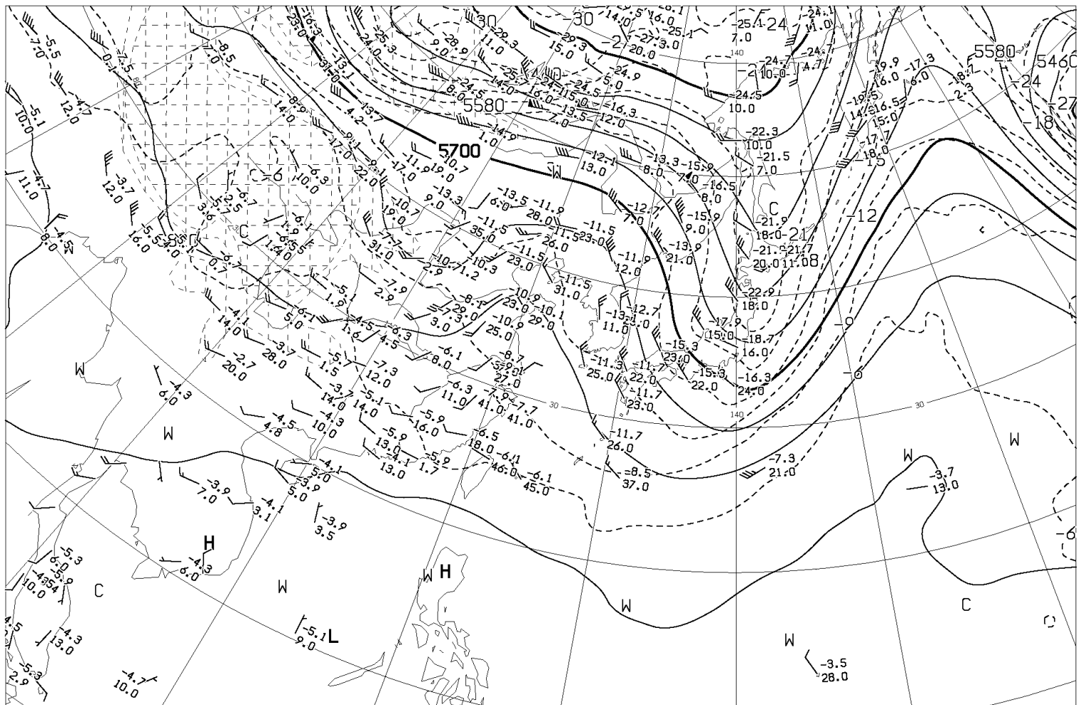
ANALYSIS 500hPa: HEIGHT(M), TEMP(°C)
