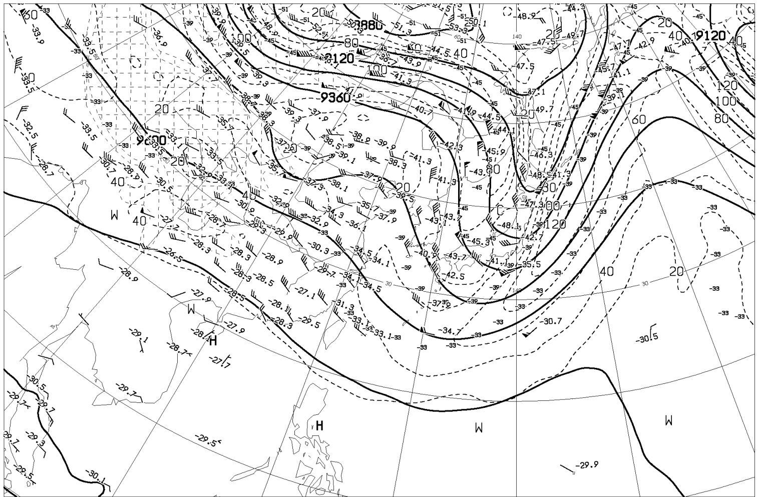
ANALYSIS 300hPa: HEIGHT(M), TEMP(°C), ISOTACH(KT)
