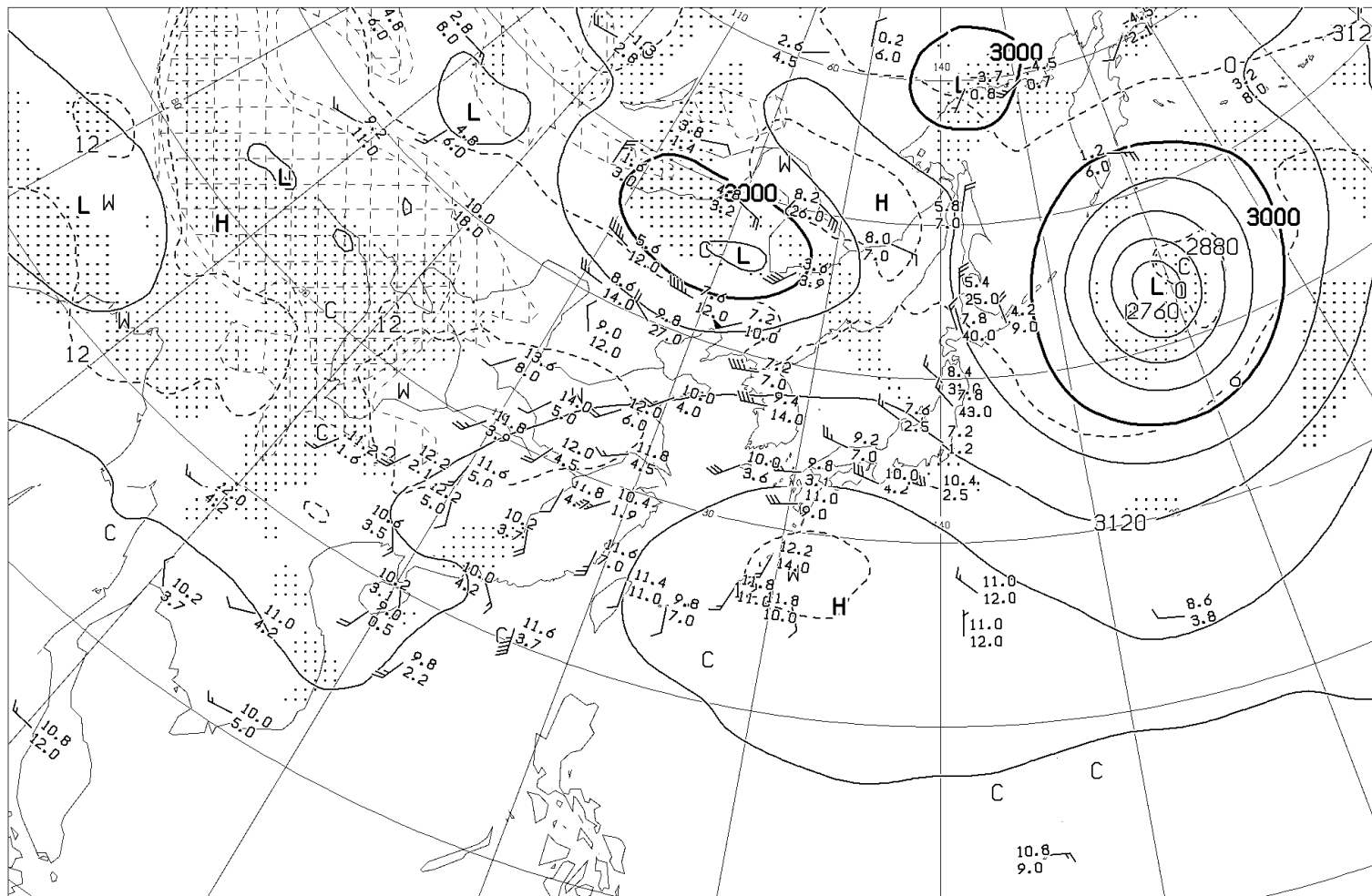
ANALYSIS 700hPa: HEIGHT(M), TEMP( ^{\circ}C ), WET AREA::( T-TD<3^{\circ}C )
