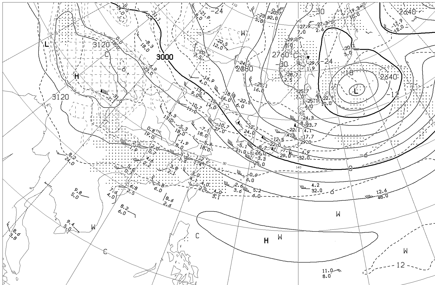
ANALYSIS 700hPa: HEIGHT(M), TEMP(°C), WET AREA::( T-TD<3^{\circ}C )
