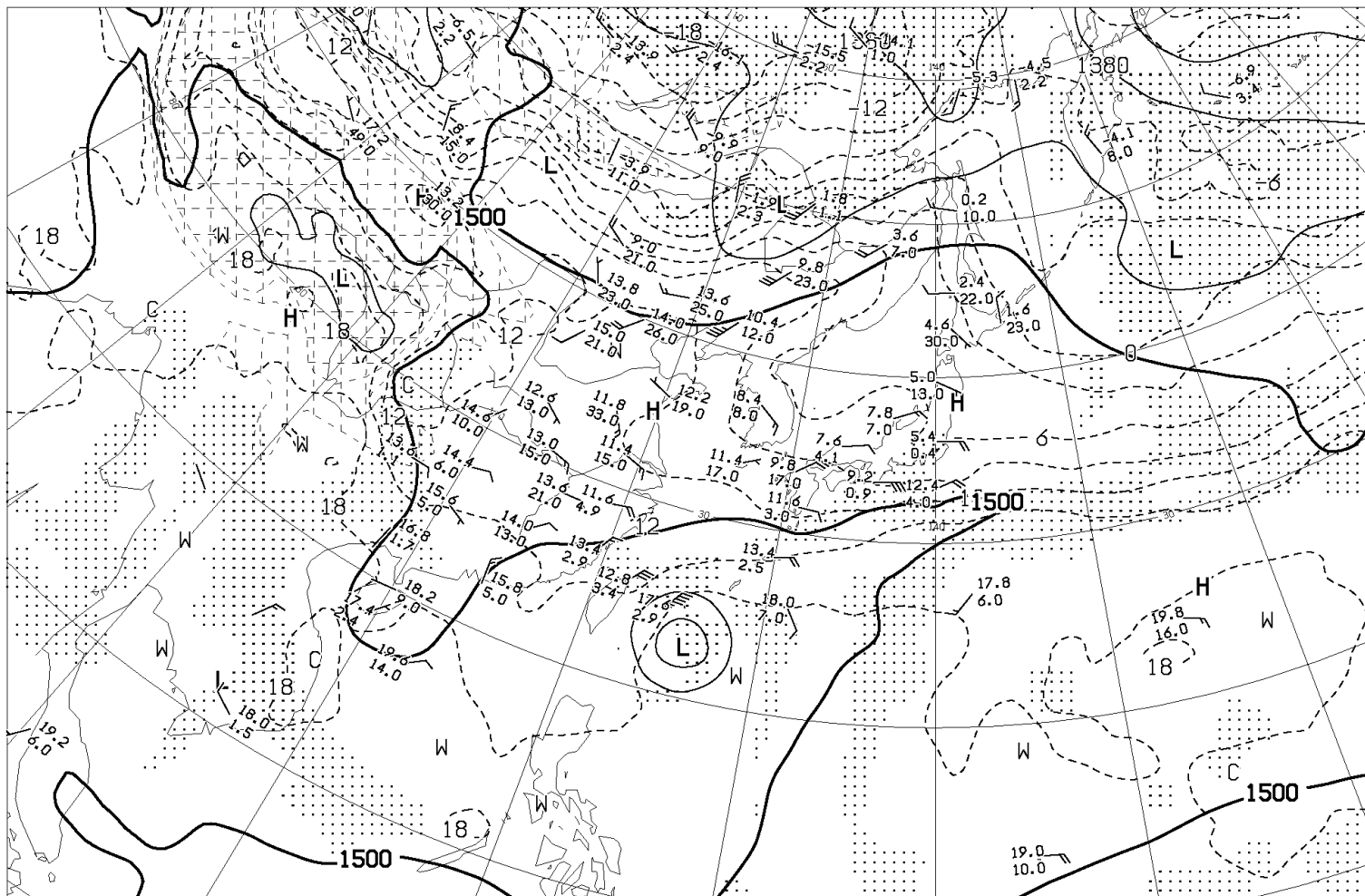
ANALYSIS 850hPa: HEIGHT(M), TEMP(°C), WET AREA::( T-TD<3^{\circ}\text{C} )
