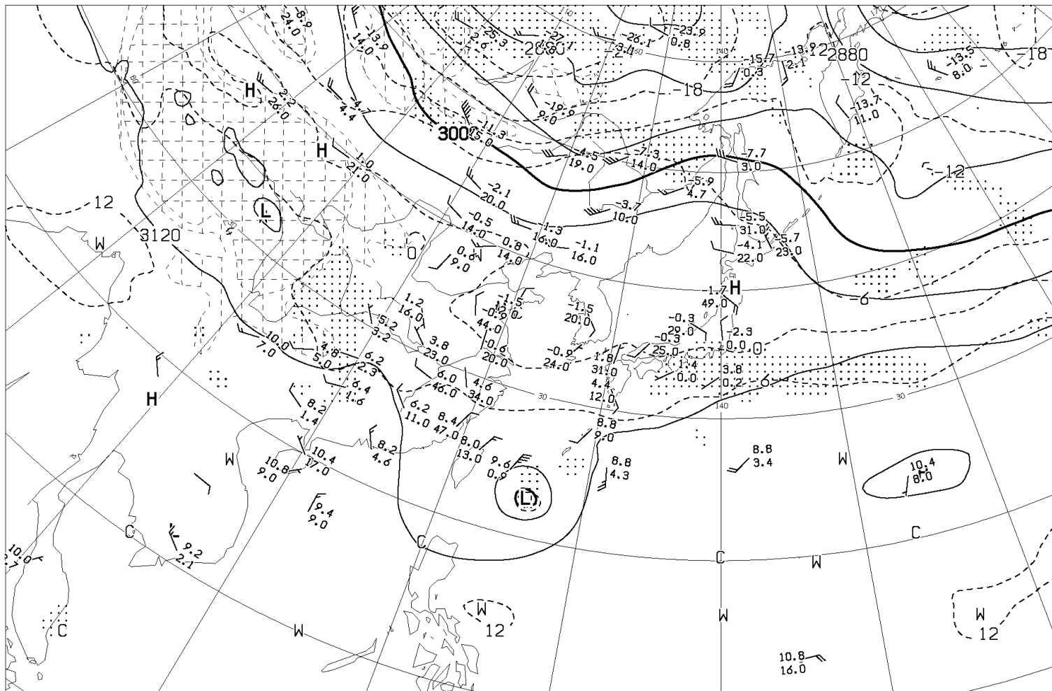
ANALYSIS 700hPa: HEIGHT(M), TEMP(°C), WET AREA::( T-TD<3^{\circ}\text{C} )
