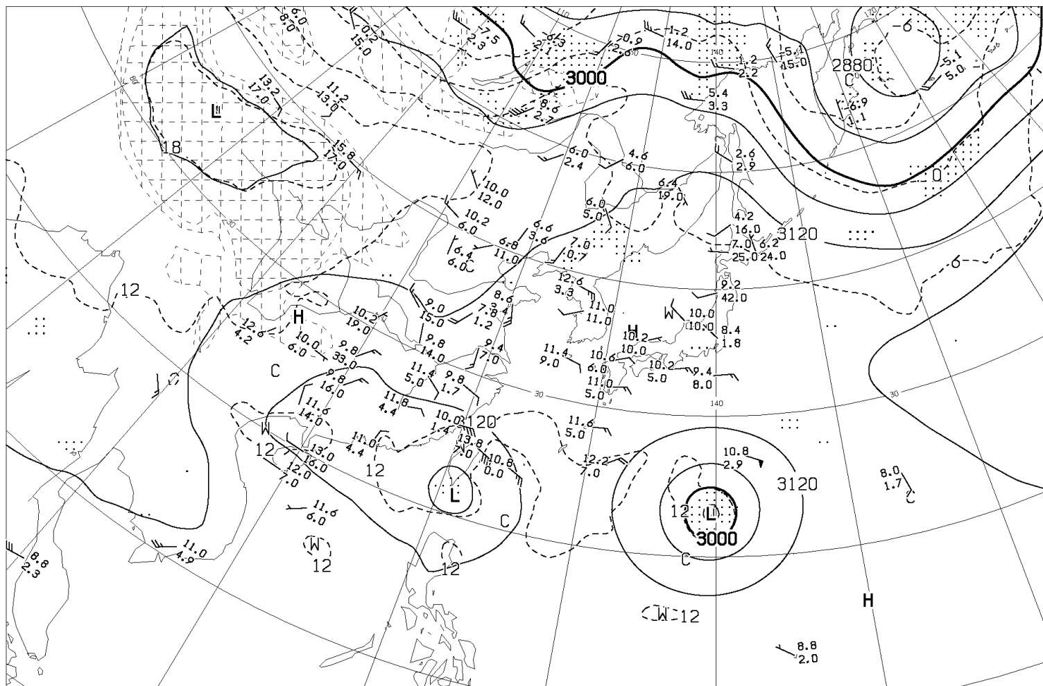
ANALYSIS 700hPa: HEIGHT(M), TEMP(°C), WET AREA::( T-TD<3^{\circ}C )
