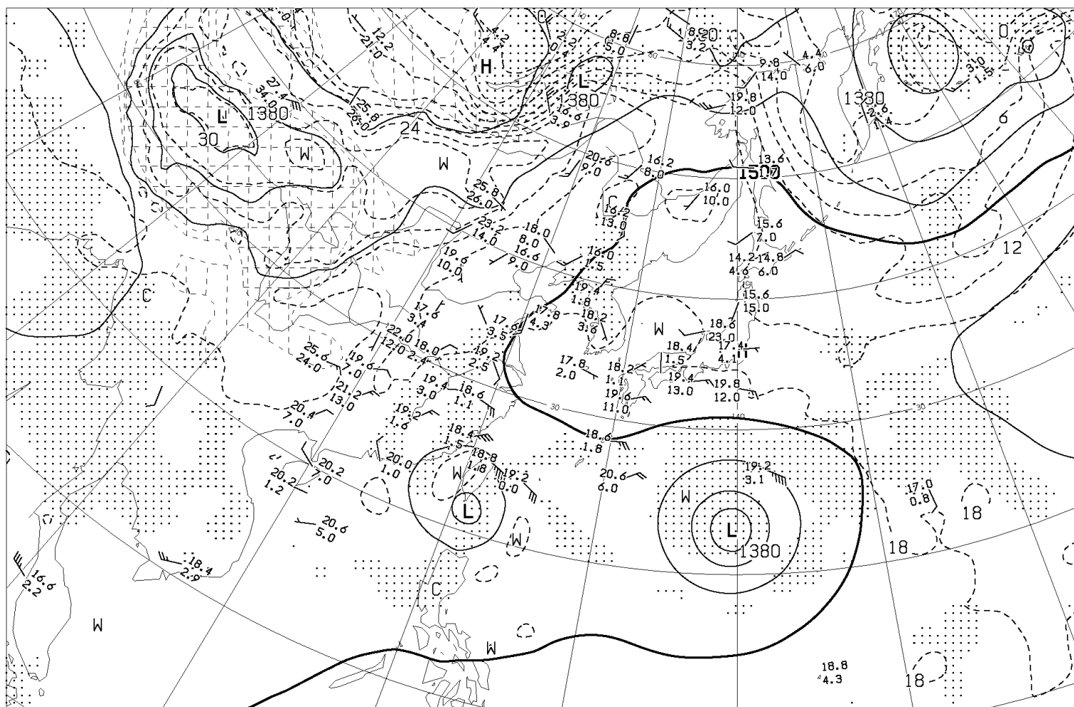
ANALYSIS 850hPa: HEIGHT(M), TEMP(°C), WET AREA::( T-TD<3^{\circ}C )
