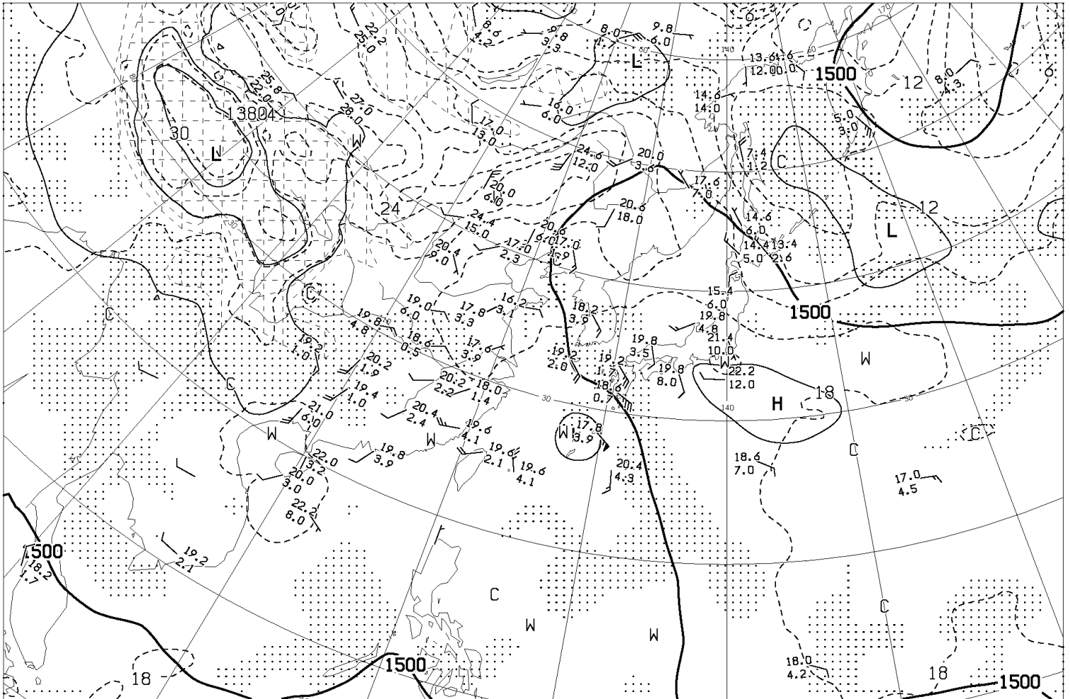
ANALYSIS 850hPa: HEIGHT(M), TEMP( ^{\circ}C ), WET AREA::( T-TD < 3^{\circ}C )
