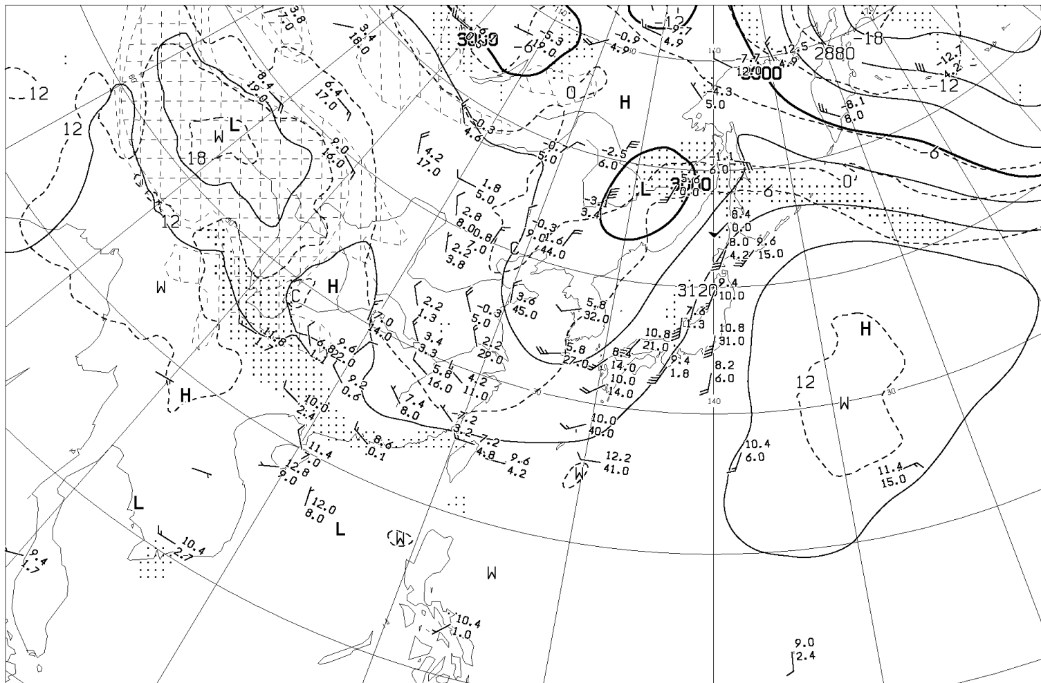
ANALYSIS 700hPa: HEIGHT(M), TEMP(°C), WET AREA::( T - TD < 3^{\circ}C )
