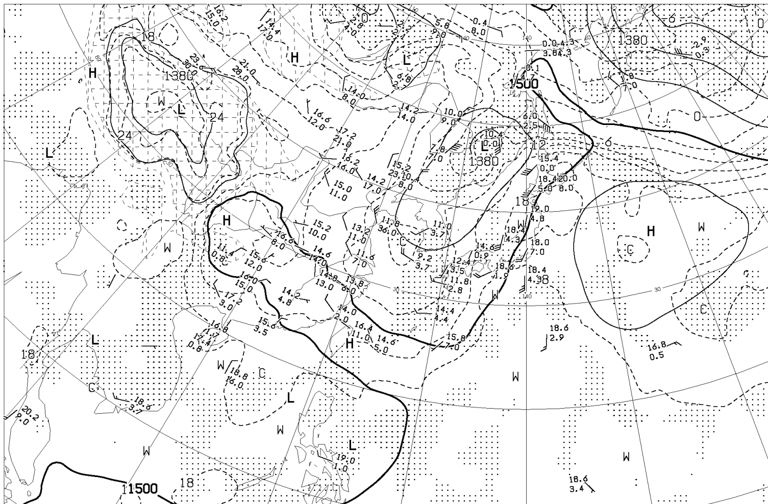
ANALYSIS 850hPa: HEIGHT(M), TEMP(°C), WET AREA::( T - TD < 3^{\circ}C )
