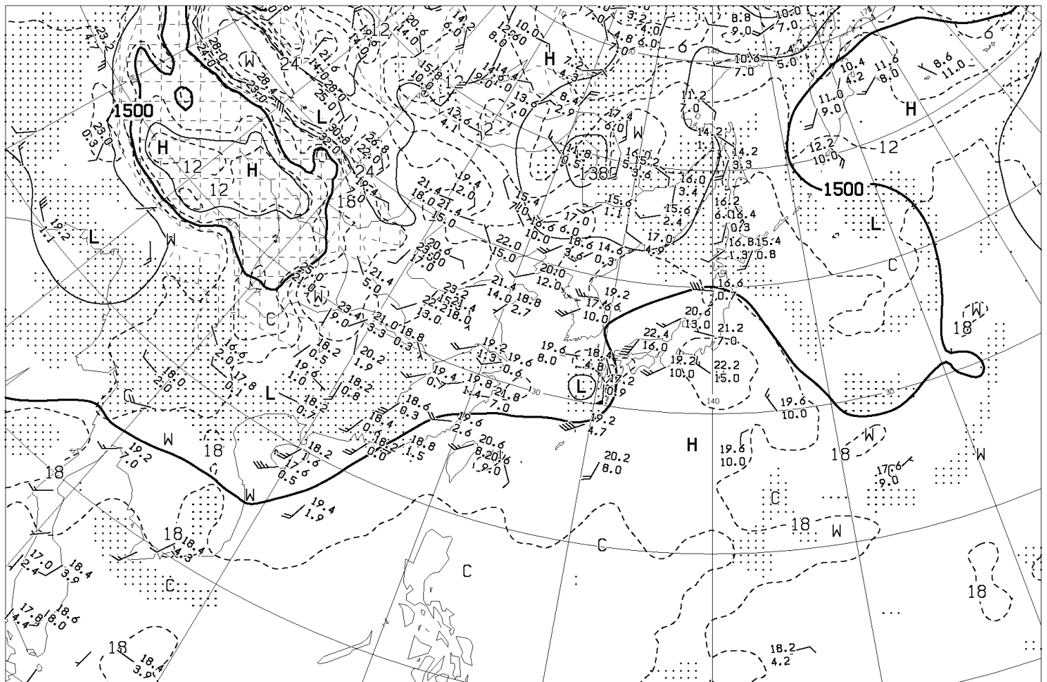
ANALYSIS 850hPa: HEIGHT(M), TEMP(°C), WET AREA::( T - TD < 3^{\circ}\text{C} )
