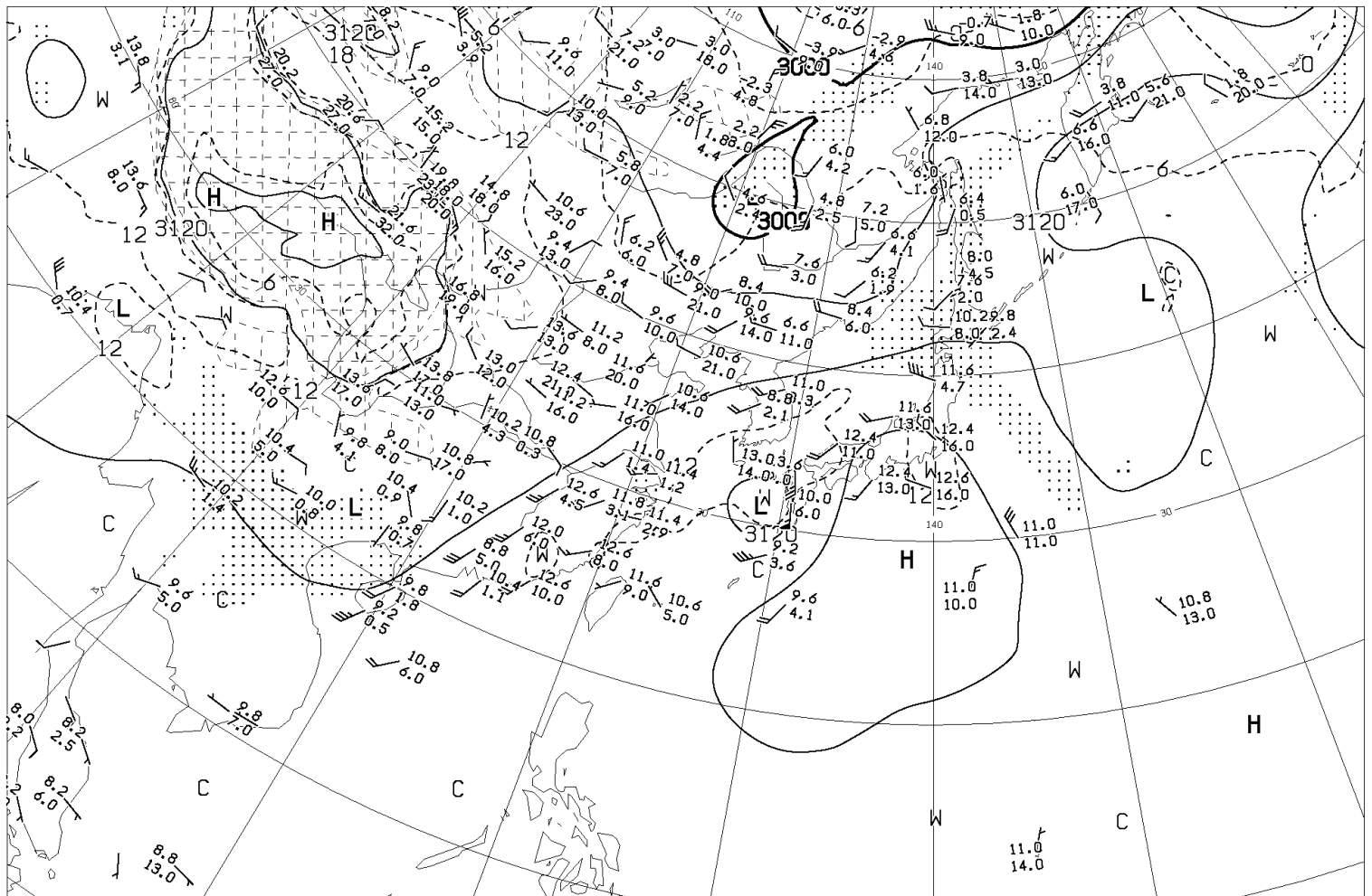
ANALYSIS 700hPa: HEIGHT(M), TEMP(°C), WET AREA::( T - TD < 3^{\circ}\text{C} )
