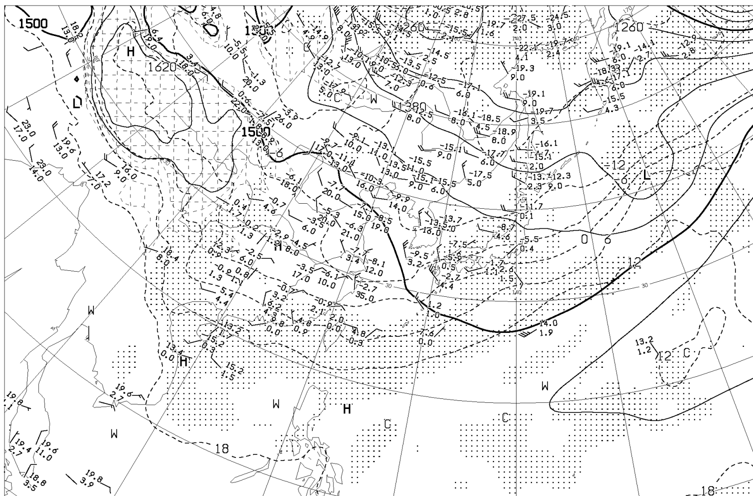
ANALYSIS 850hPa: HEIGHT(M), TEMP(°C), WET AREA::( T-TD<3^{\circ}\text{C} )
