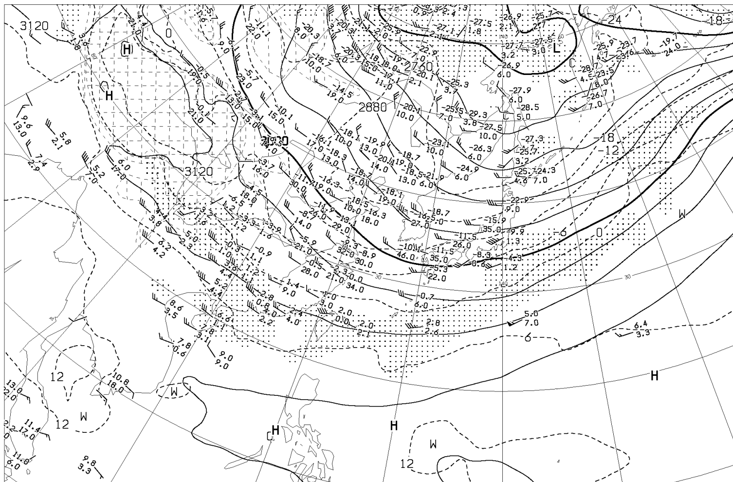
ANALYSIS 700hPa: HEIGHT(M), TEMP(°C), WET AREA::( T-TD<3^{\circ}\text{C} )
