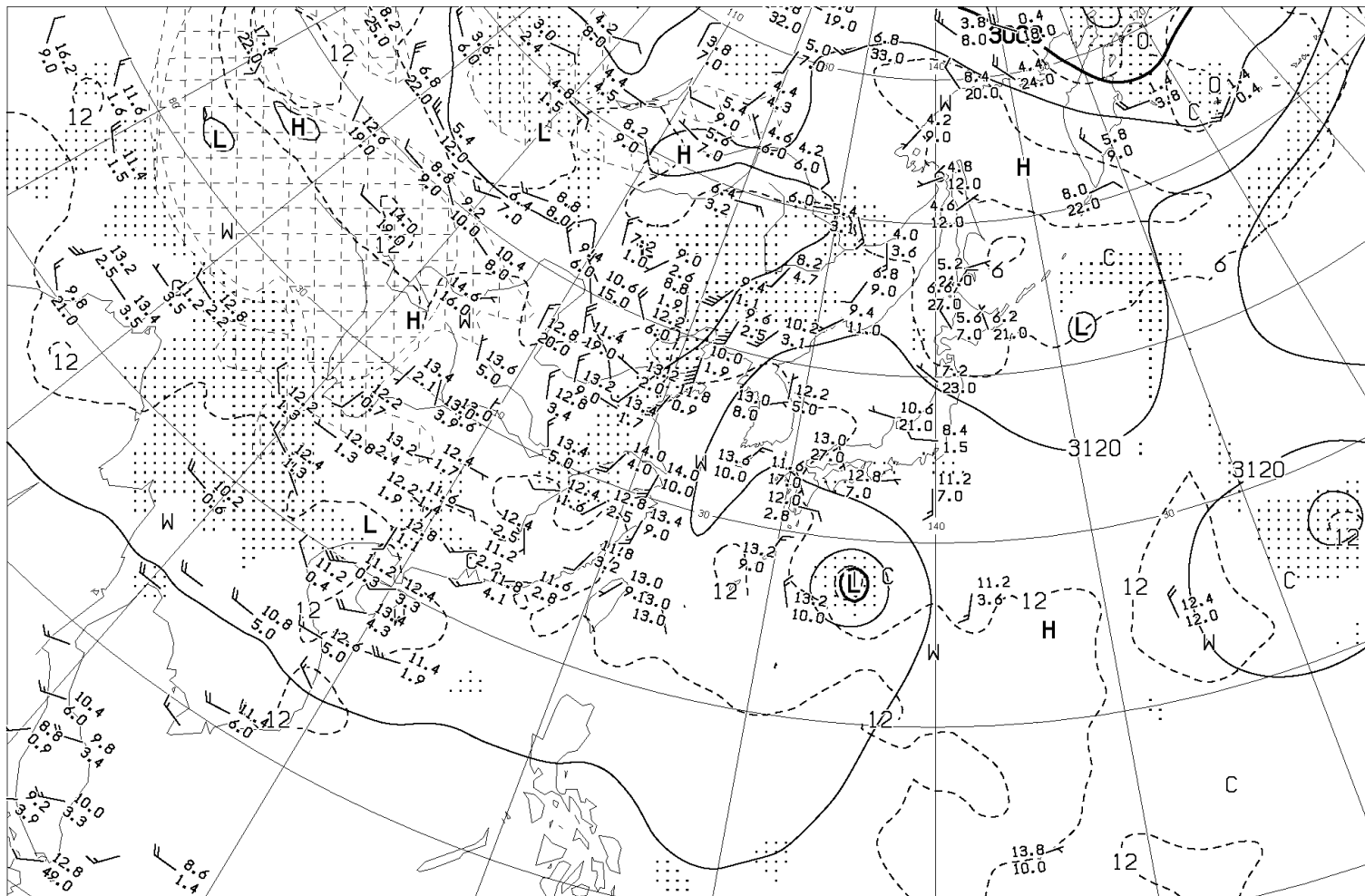
ANALYSIS 700hPa: HEIGHT(M), TEMP(°C), WET AREA::( T - TD < 3^{\circ}\text{C} )
