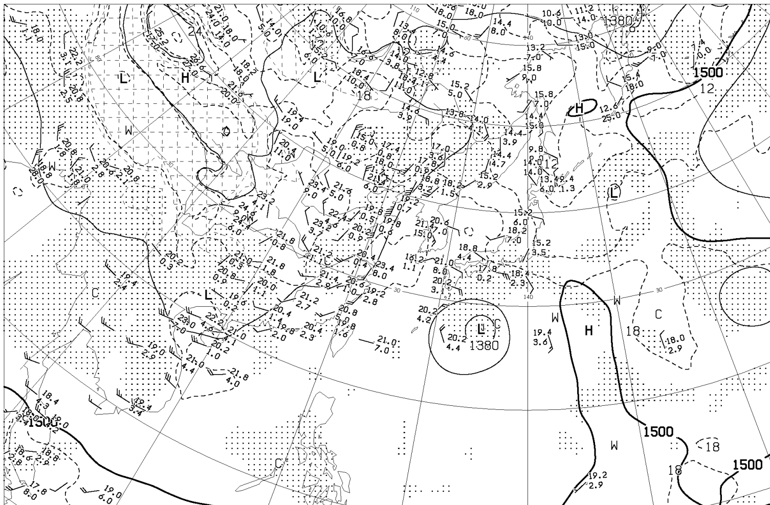
ANALYSIS 850hPa: HEIGHT(M), TEMP(°C), WET AREA::( T - TD < 3^{\circ}\text{C} )
