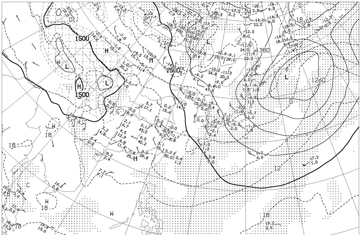
ANALYSIS 850hPa: HEIGHT(M), TEMP( ^\circ\text{C} ), WET AREA::( T - T_D < 3^\circ\text{C} )
