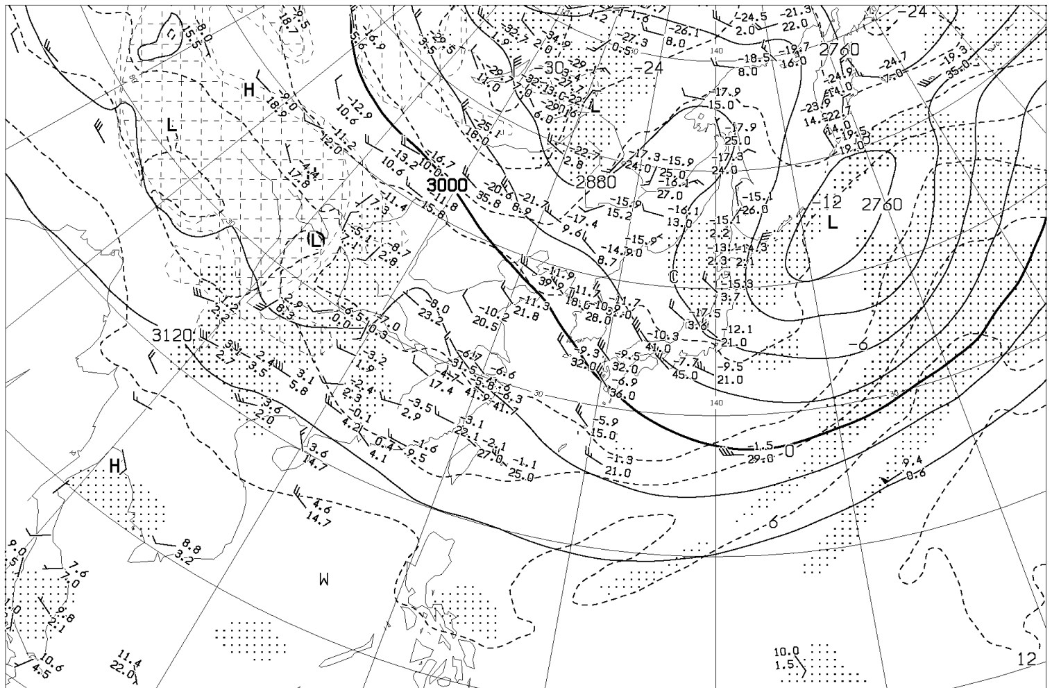
ANALYSIS 700hPa: HEIGHT(M), TEMP( ^\circ\text{C} ), WET AREA::( T - T_D < 3^\circ\text{C} )
