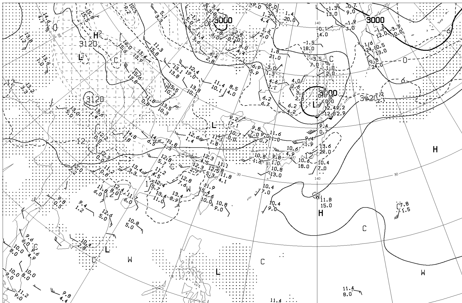
ANALYSIS 700hPa: HEIGHT(M), TEMP(°C), WET AREA::(T-12<3°C)
