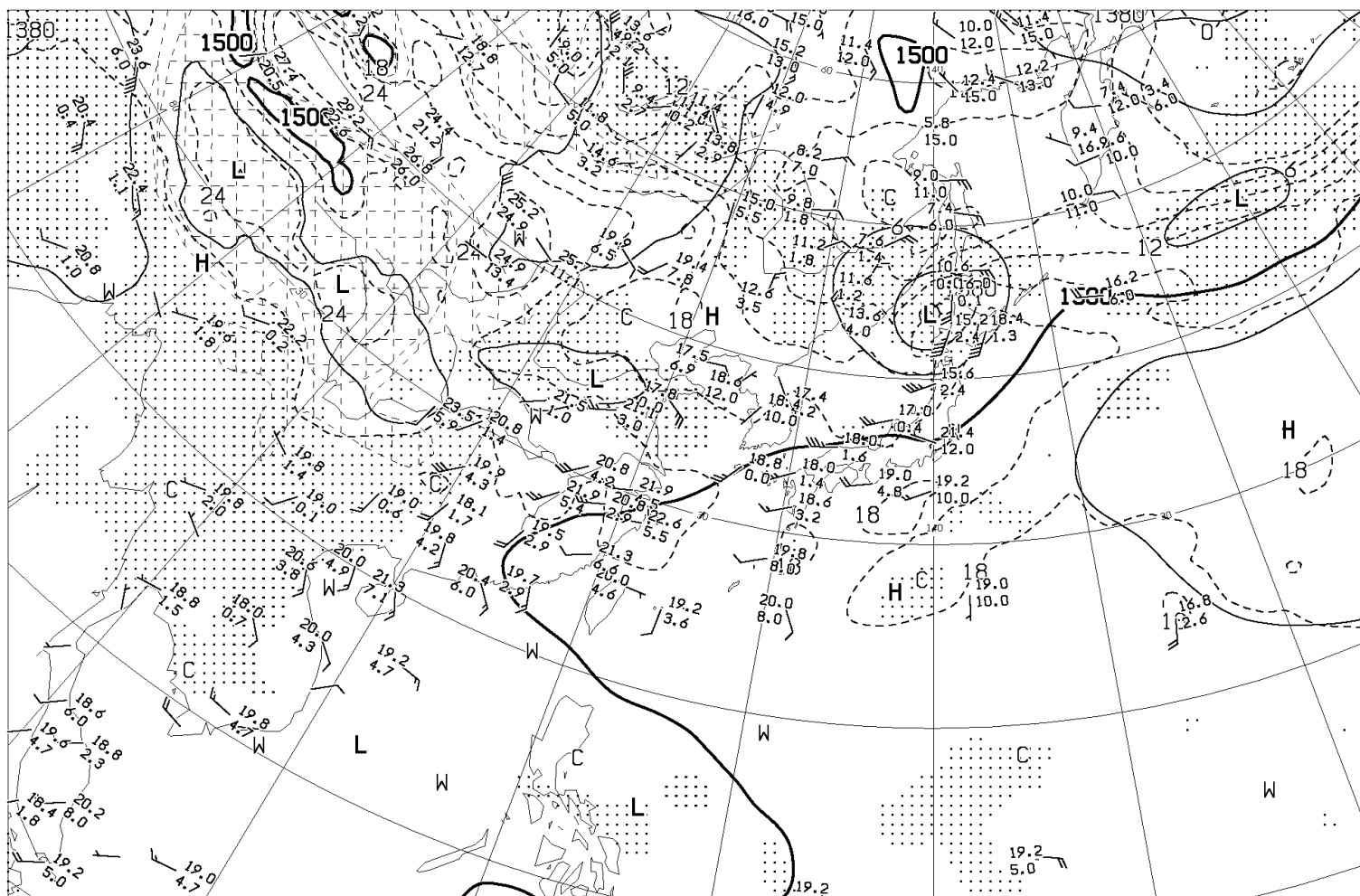
ANALYSIS 850hPa: HEIGHT(M), TEMP(°C), WET AREA::(T-12<3°C)
