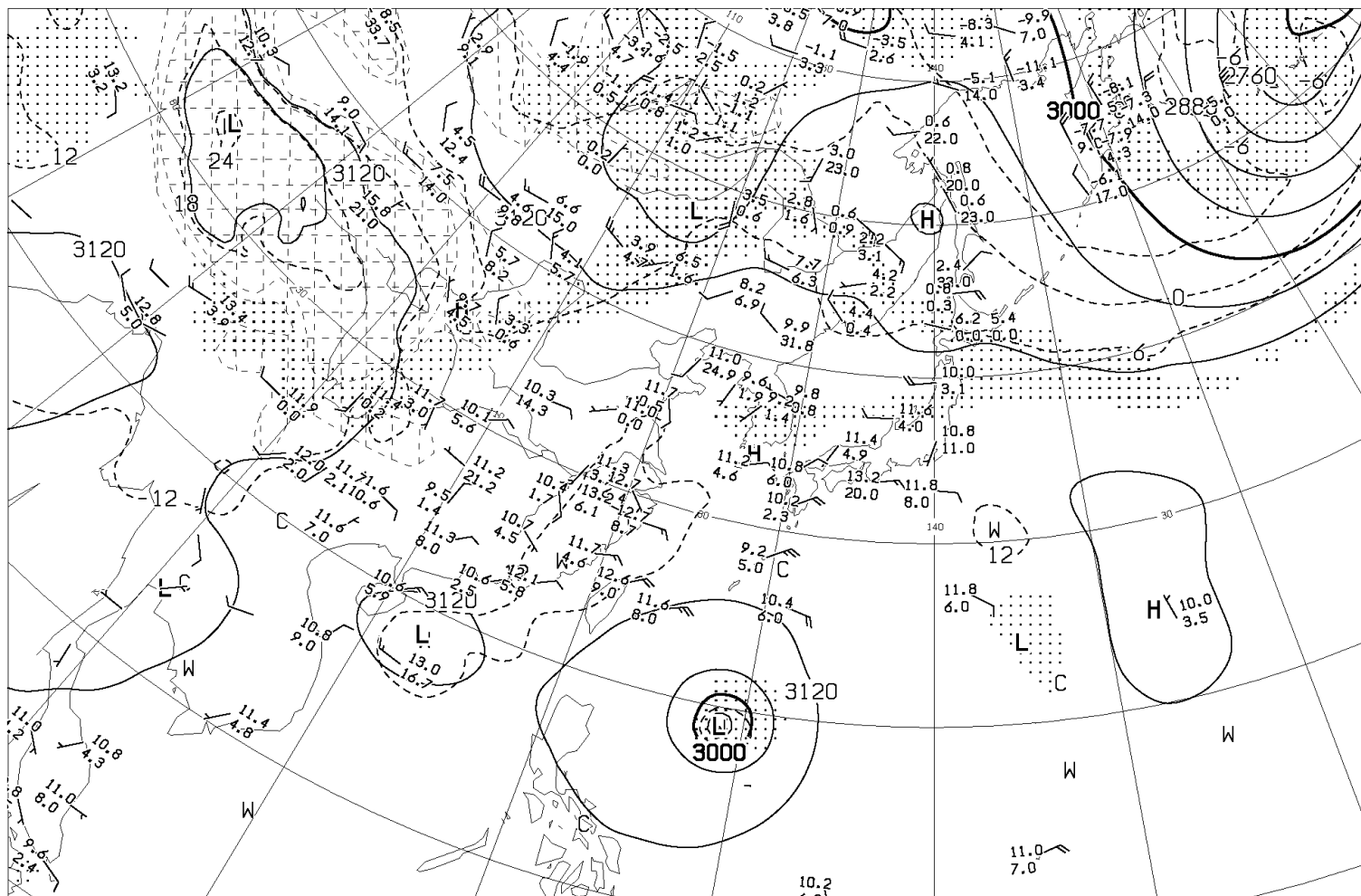
ANALYSIS 700hPa: HEIGHT(M), TEMP(°C), WET AREA::(T-T 2 <3°C)
