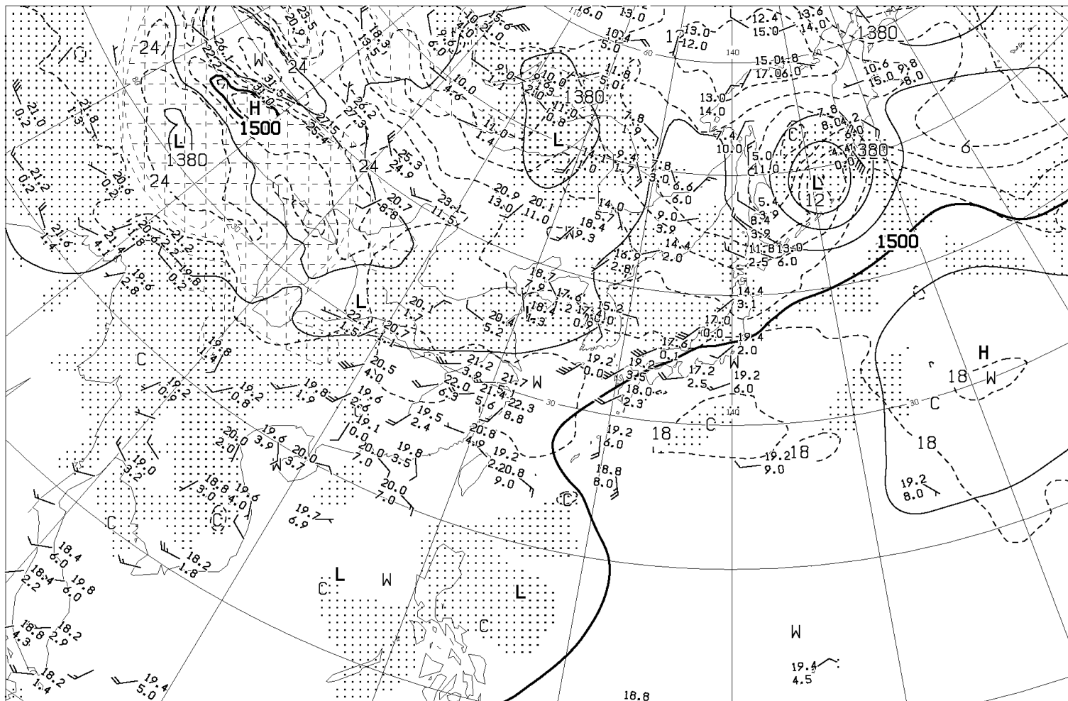
ANALYSIS 850hPa: HEIGHT(M), TEMP(°C), WET AREA::(T-ID*3°C)
