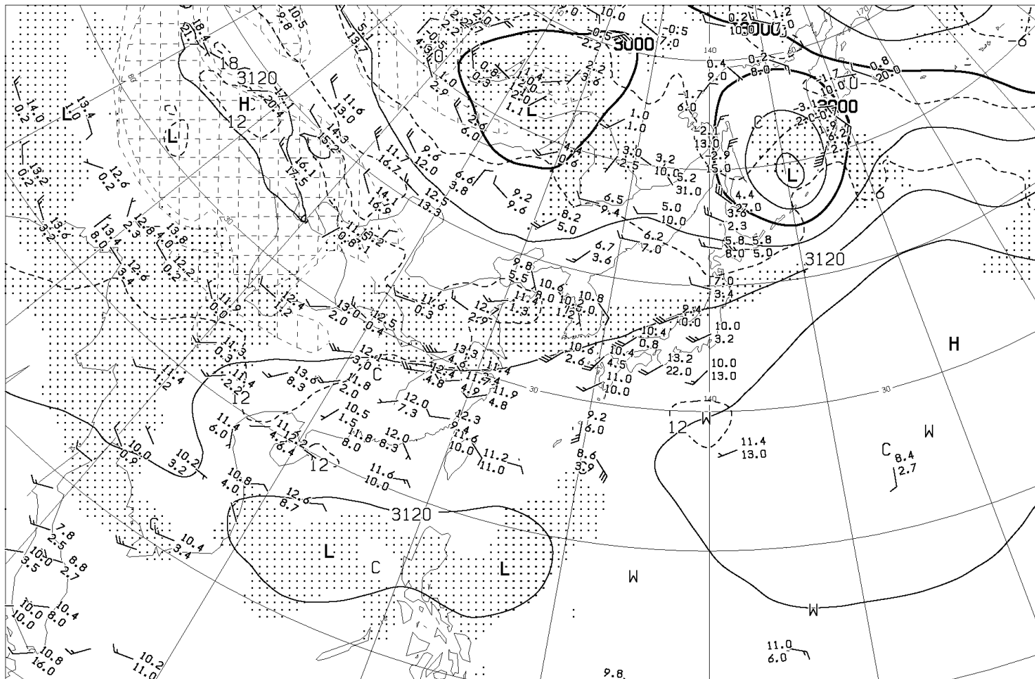
ANALYSIS 700hPa: HEIGHT(M), TEMP(°C), WET AREA::(T-ID*3°C)
