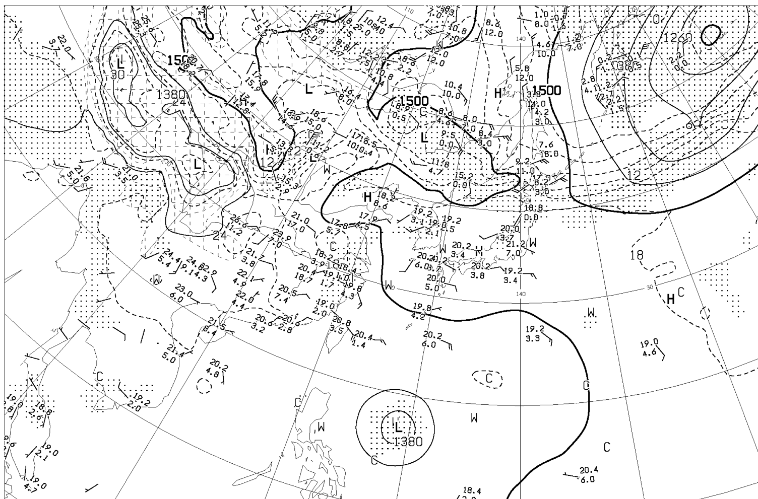
ANALYSIS 850hPa: HEIGHT(M), TEMP(°C), WET AREA:: (T-ID<3°C)
