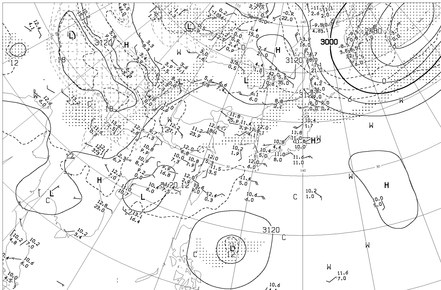
ANALYSIS 700hPa: HEIGHT(M), TEMP(°C), WET AREA:: (T-ID<3°C)
