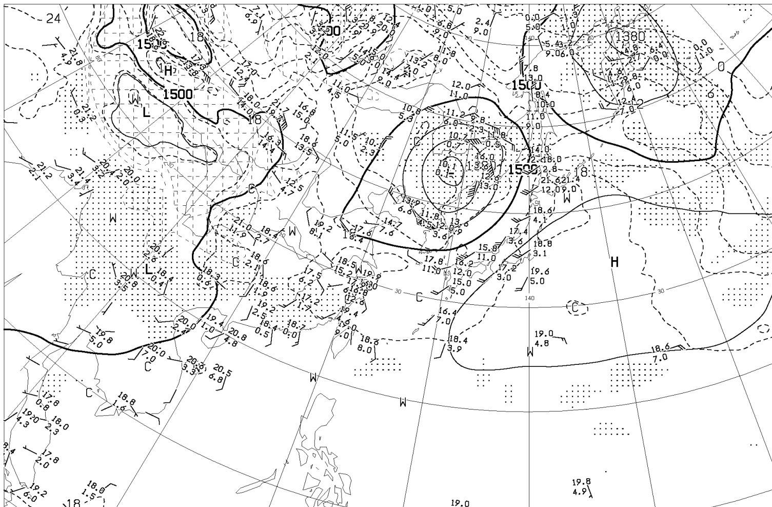
ANALYSIS 850hPa: HEIGHT(M), TEMP(°C), WET AREA::( T-ID < 3^{\circ}C )
