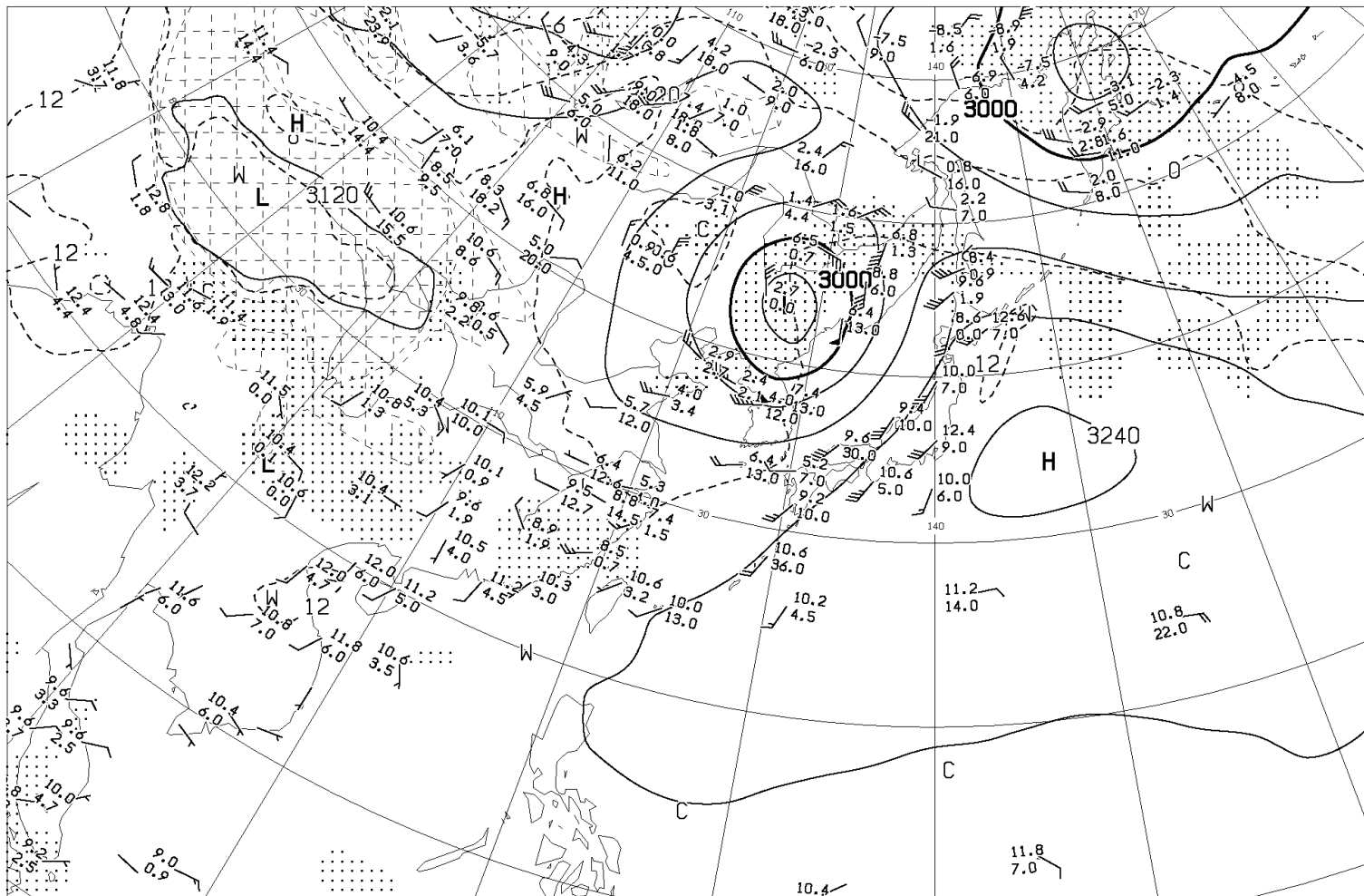
ANALYSIS 700hPa: HEIGHT(M), TEMP(°C), WET AREA::( T-ID < 3^{\circ}C )
