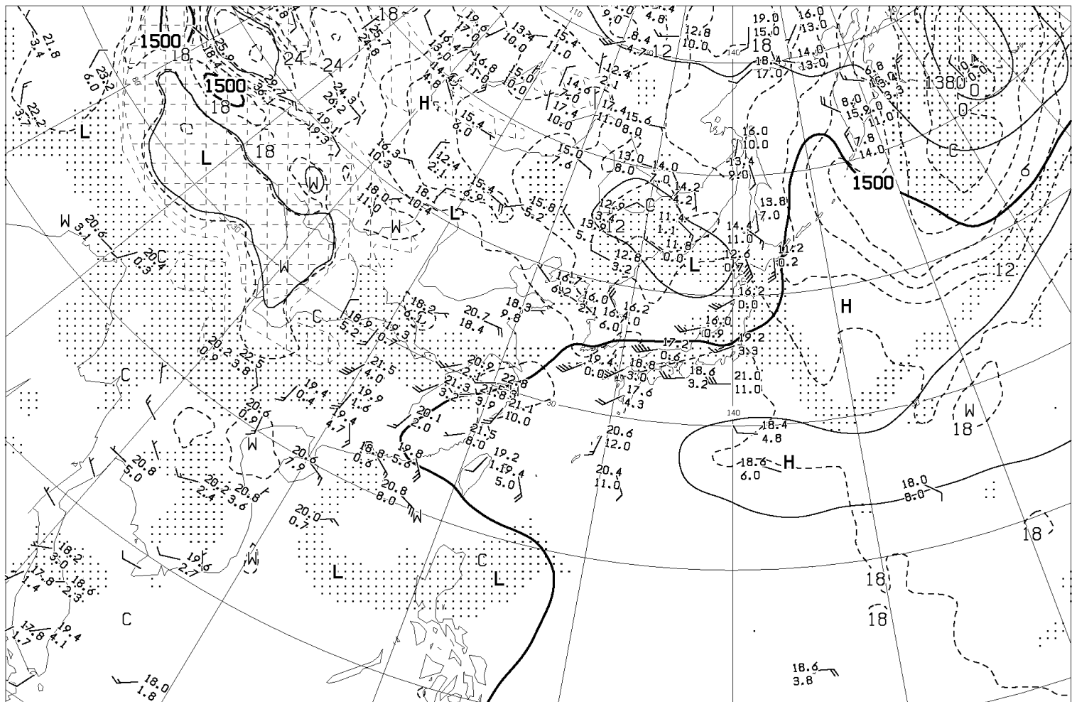
ANALYSIS 850hPa: HEIGHT(M), TEMP(°C), WET AREA::(T-TD<3°C)
